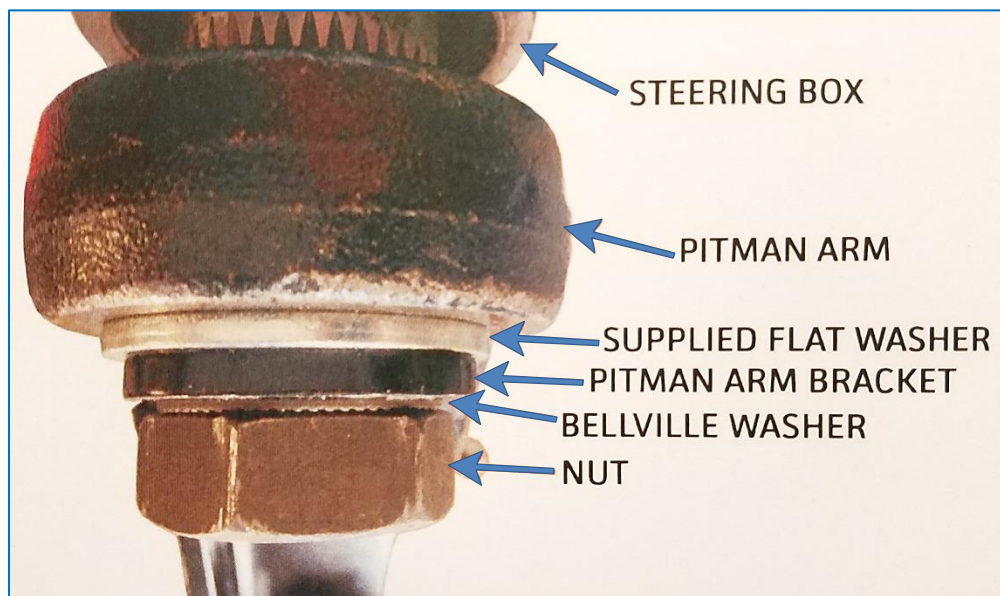
Pitman Arm FIG. A
